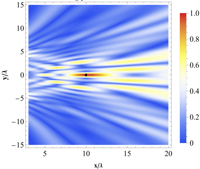
Beam focusing pattern for Modular ULA
